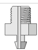
130.194 G 1/4"AG
